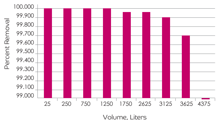
Average Legionella Removal and Capacity for Disruptor® Media with Prefilter
