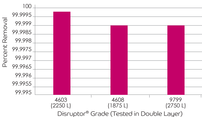
Percent Removal of Legionella at Disruptor® Filter Capacity
